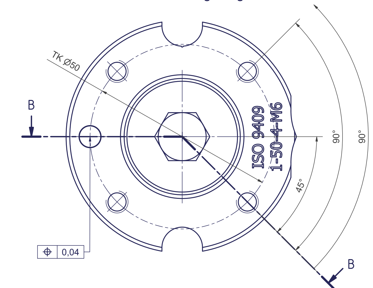
A (2 : 1) Tool mounting flange
