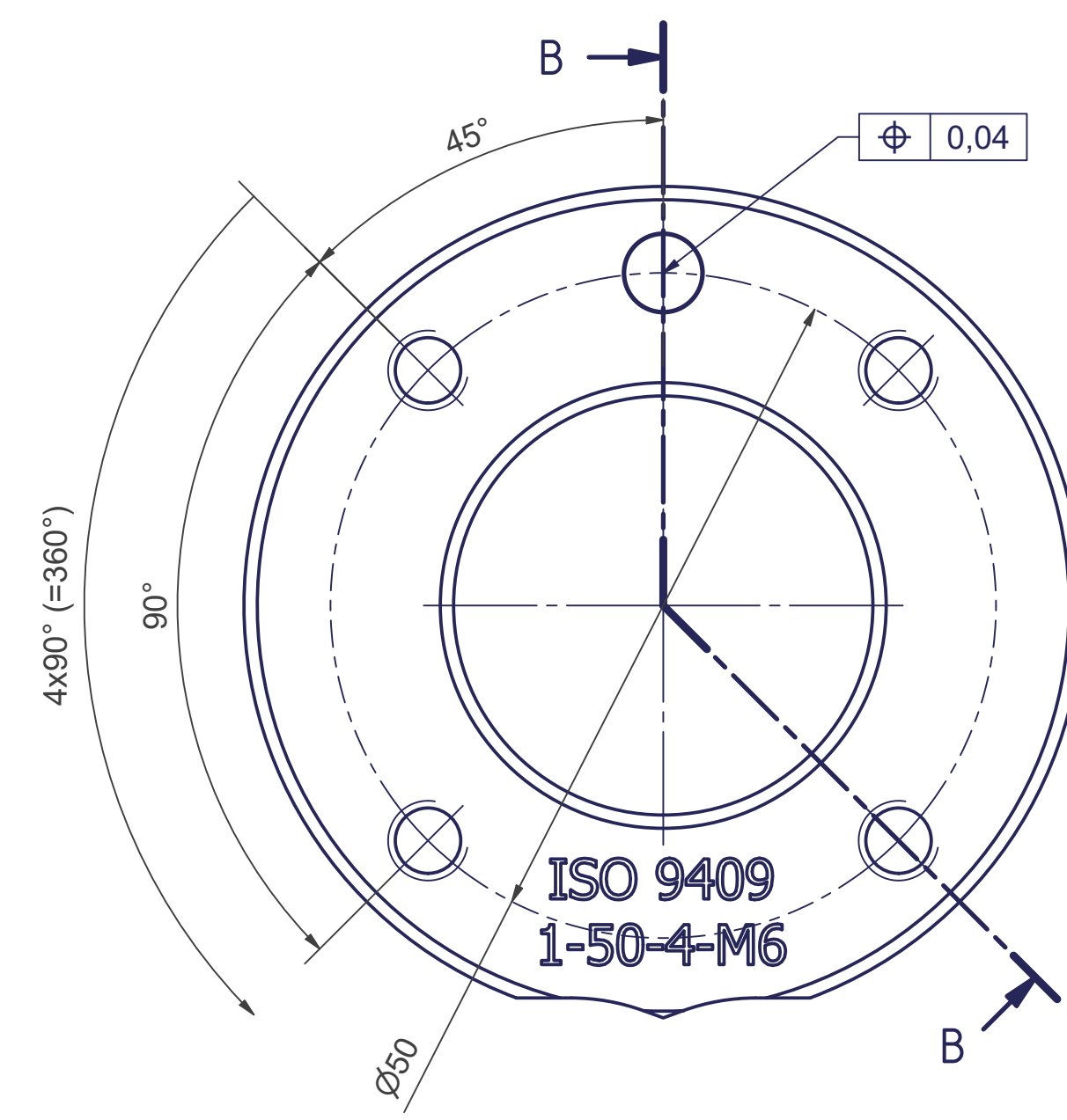
A (2 : 1) Tool mounting flange
